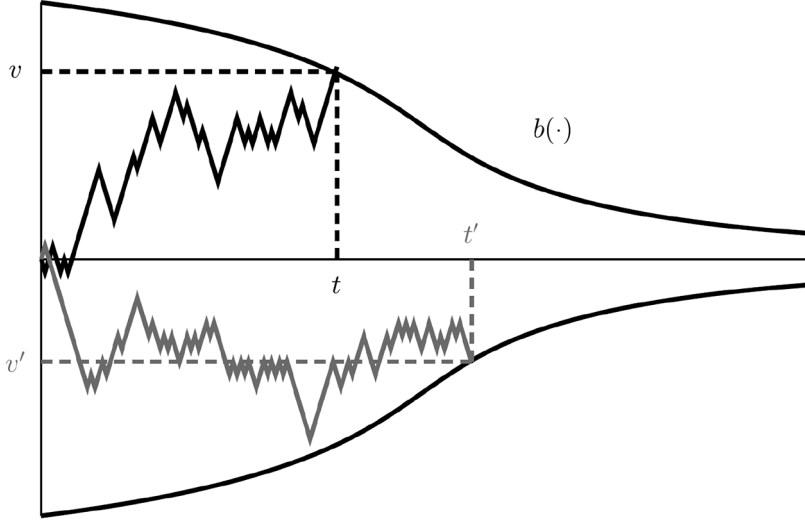
FIG. 2.—Illustration of a DDM with collapsing decision boundaries.
