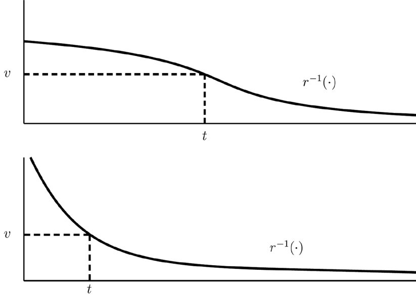
FIG. 1.—Two illustrations of chronometric functions r , mapping realized utility differences (vertical axis) into response times (horizontal axis).
